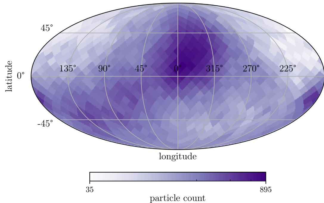
Dark matter halo
