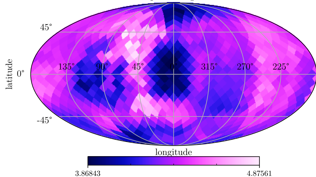
Bound neutrino percentage of m_\nu = 0.1 eV
